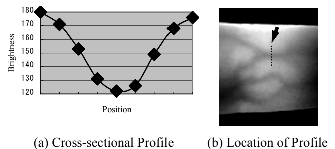
Fig. 6 Cross-sectional Profile of Finger Vein Image
