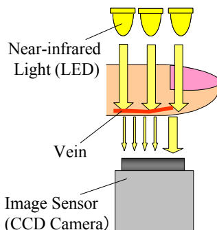
Fig. 2 Light Transmission Method
